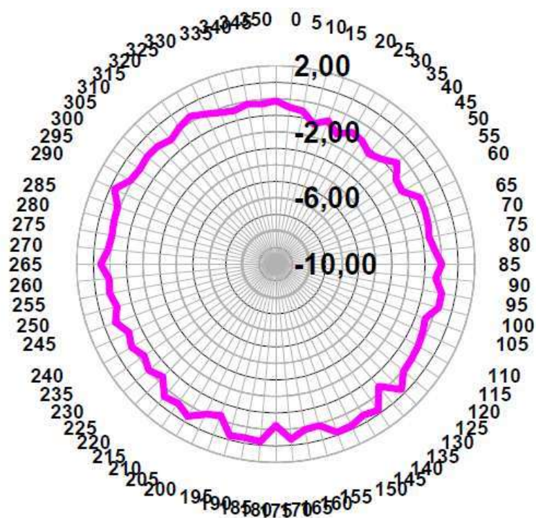
Freq. 1800 MHz H-plane (dBi) V-pol
